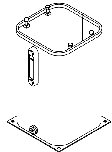
ISOMETRIC VIEW SCALE 1 : 8
